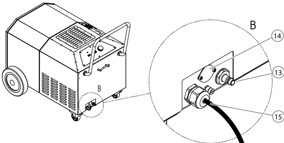
Abb. 2: Anschlüsse
